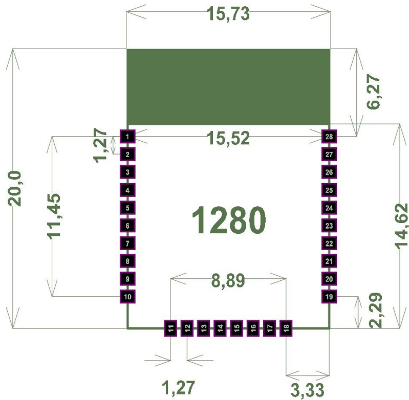
Figure 3: EMB-LR1280S suggested footprint
